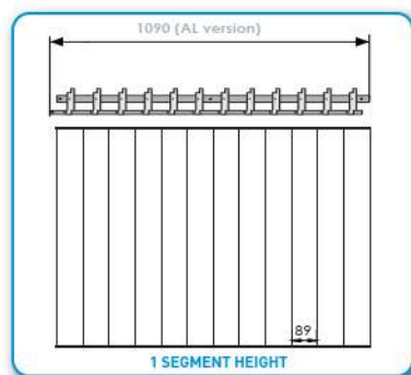
1 SEGMENT HEIGHT
