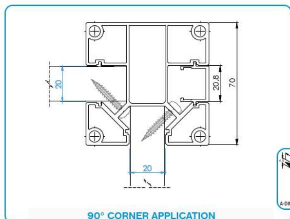
90° CORNER APPLICATION
